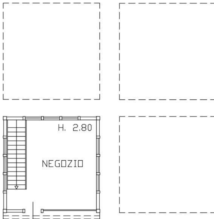
PIANO TERRA
